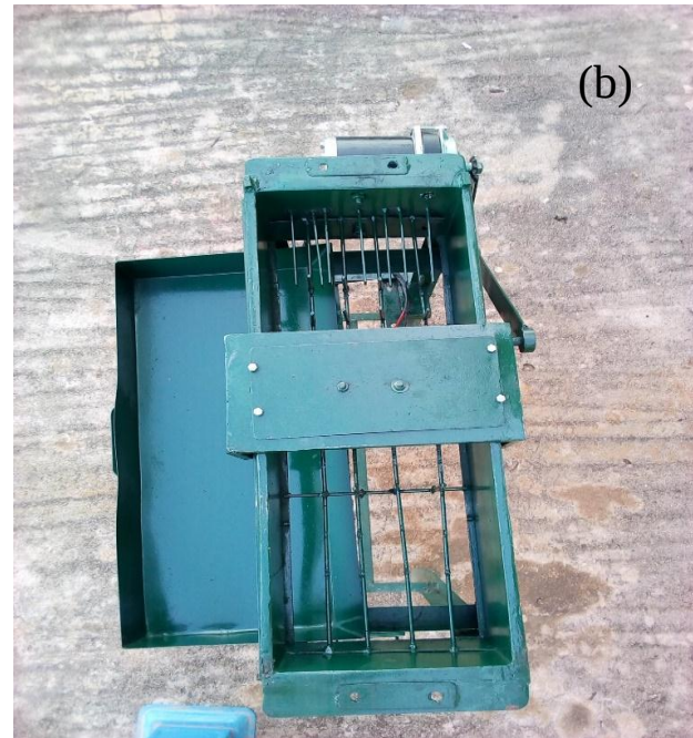
Fig 1. (a) Isometric View of Cucumber Slicing Machine; (b) Constructed Cucumber Slicing Machine.
